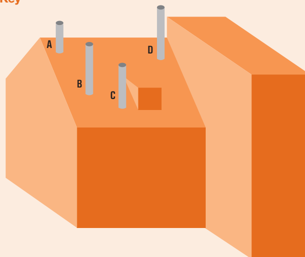
Diagram 4 - Typical flue outlet positions for a traditional roof as shown in Approved Document J
