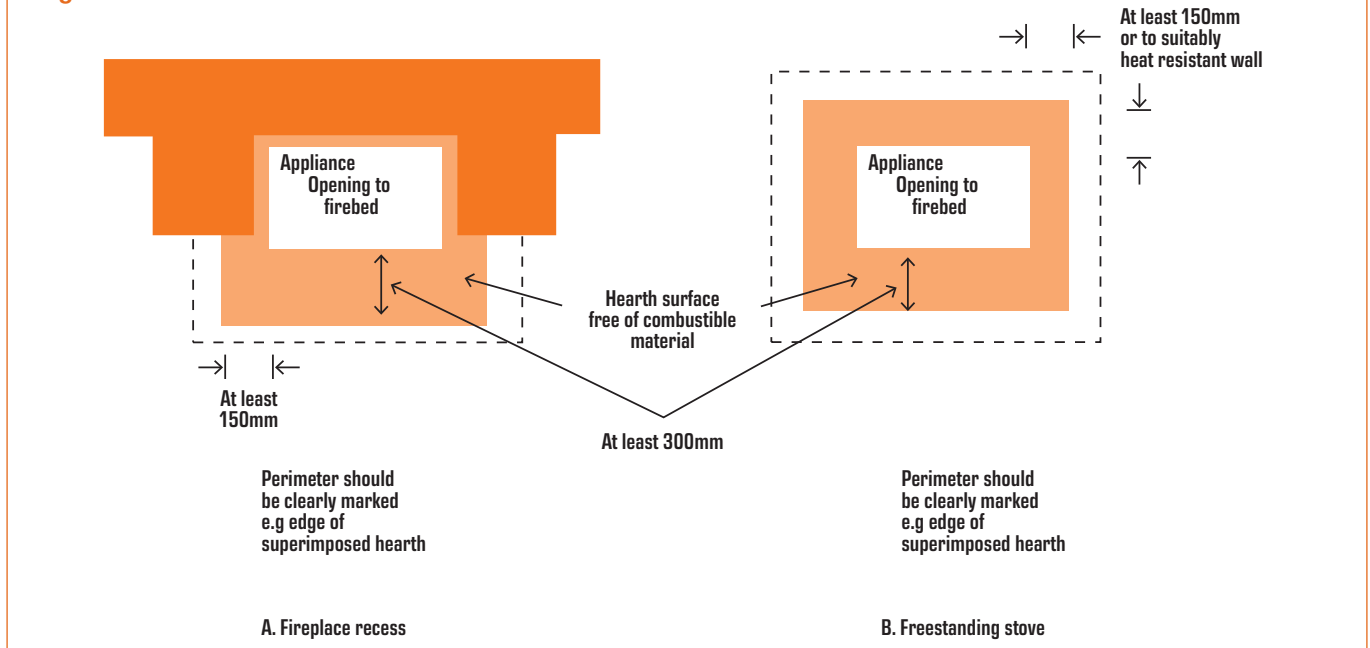
Diagram 5 - Hearth sizes
