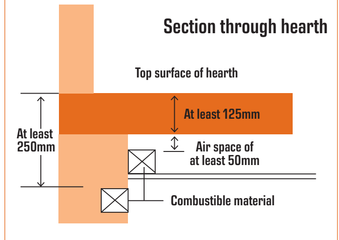
Diagram 6 - Hearth thickness
