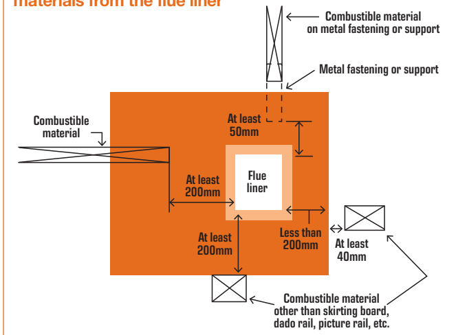
Diagram 3 - Chimneys; Separating combustible materials from the flue liner
