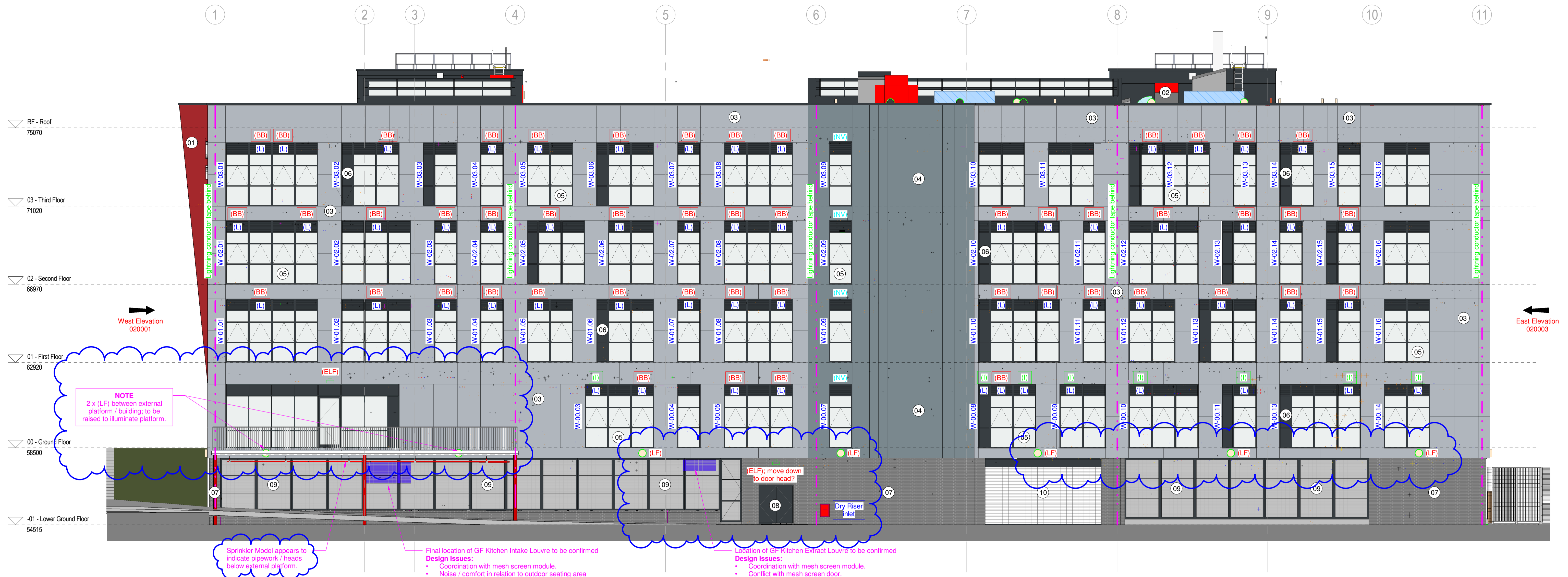
1- Proposed South Elevation - GA Scale: 1 : 100
